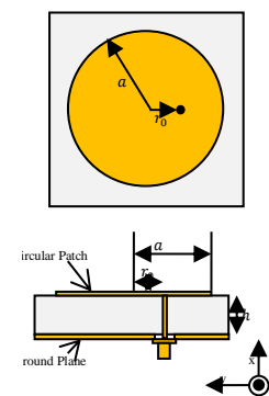
Figure 1. Geometry of circular microstrip antenna.
