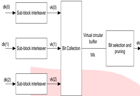
Gambar 2. Rate Matching for transport channel diadaptasi dari [3]
