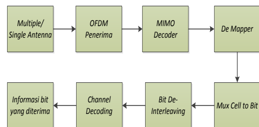
Gambar 3.5 Blok Diagram Penerima
